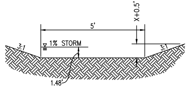
Ⓑ OPEN CHANNEL "B" CROSS SECTION
