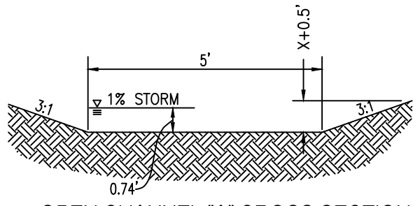
A OPEN CHANNEL "A" CROSS SECTION
