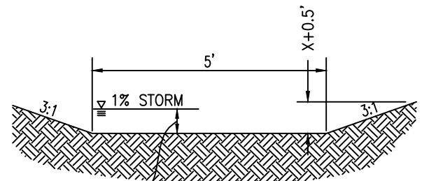
A OPEN CHANNEL "A" CROSS SECTION
