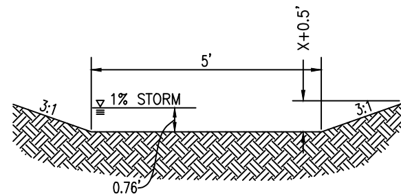
B OPEN CHANNEL "B" CROSS SECTION
