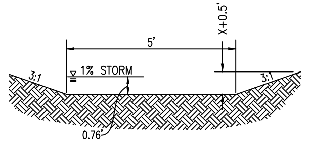
(B) OPEN CHANNEL "B" CROSS SECTION
