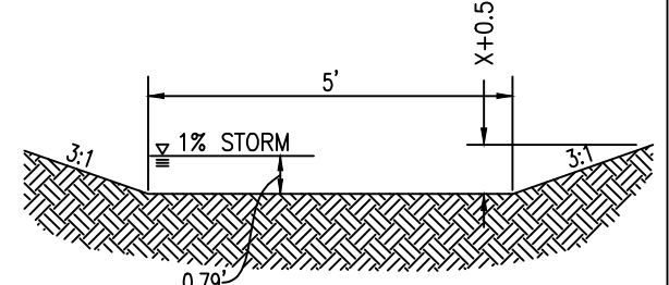
B OPEN CHANNEL "B" CROSS SECTION
