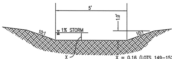
F OPEN CHANNEL "F" CROSS SECTION
