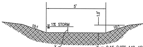
Ⓕ OPEN CHANNEL 'F' CROSS SECTION
