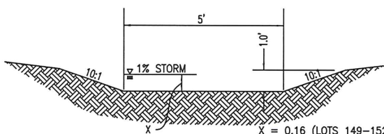
(F) OPEN CHANNEL 'F' CROSS SECTION
