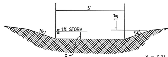
⑧ OPEN CHANNEL "B" CROSS SECTION
