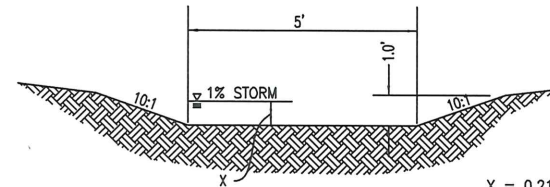
OPEN CHANNEL "B" CROSS SECTION
